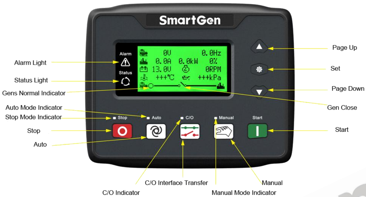
Fig.1 - HGM4010N/HGM4010NC/HGM4010CAN Front Panel Indication
