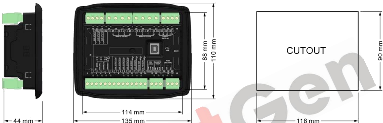
Fig.10 - Overall Dimensions
