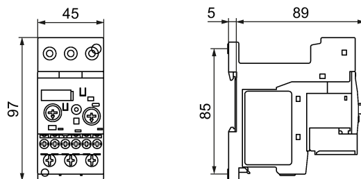
Figure C-18 3RB3.2-..B0 and 3RU2926-3AA01
