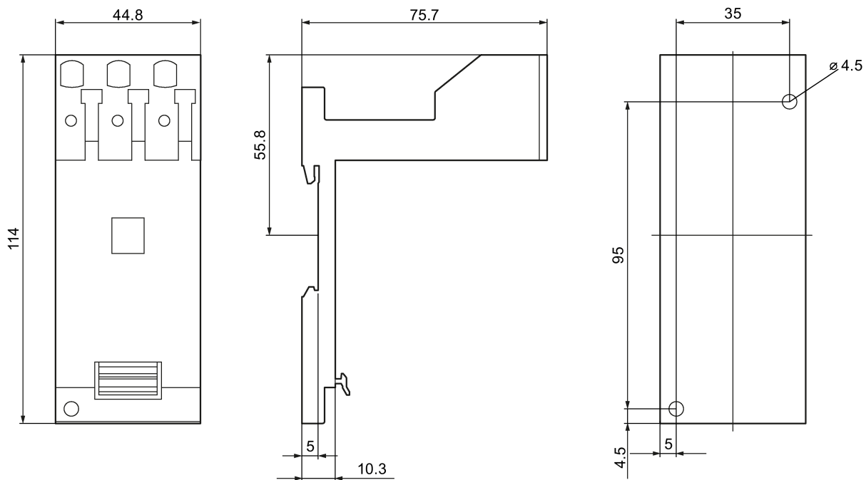
Figure C-34 3RU2926-3AC01
