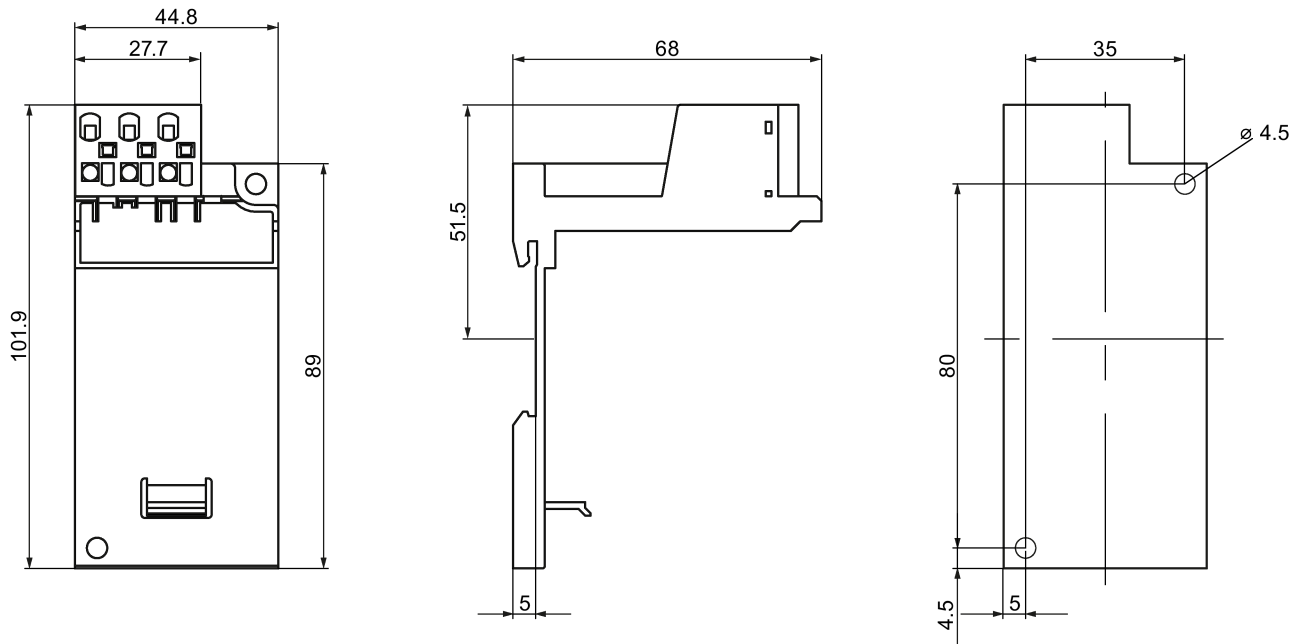
Figure C-32 3RU2916-3AC01
