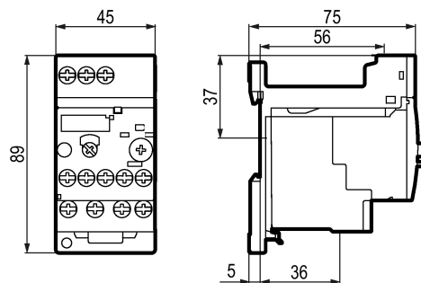
Figure C-2 3RU2116-4.B1
