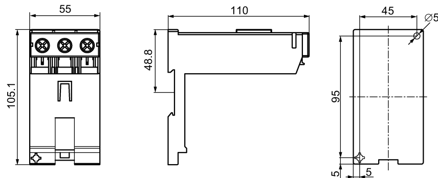
Figure C-35 3RU2936-3AA01
