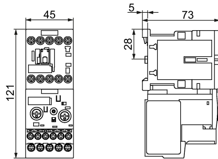
Figure C-13 3RB3.1-..B0
