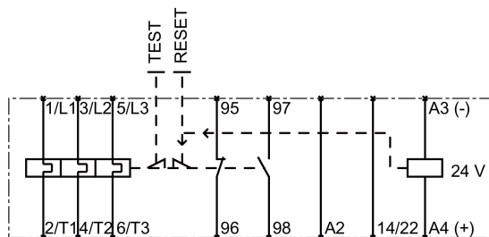
Figure 12-10 3RB31 solid-state overload relay, screw-type connection system, S00
