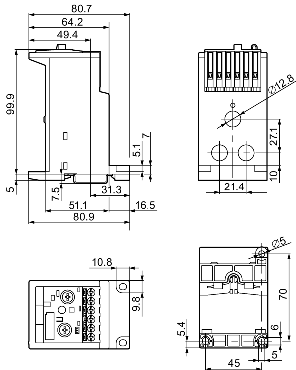
Figure C-25 3RB3.3-..W.
